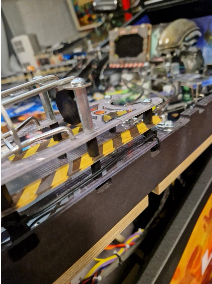
Step 8: Install new right side orbit plastic with flasher.
